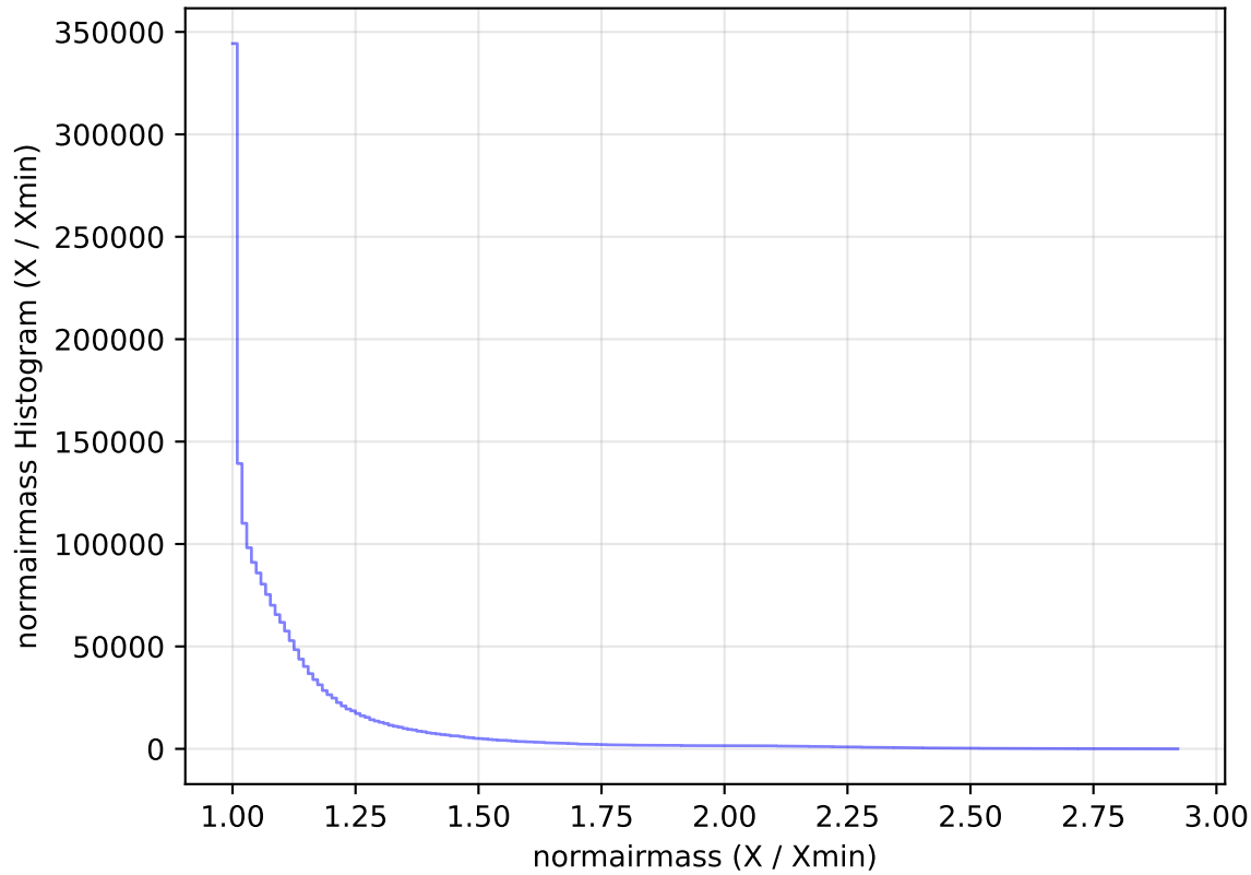
internal_u_expt27_nscale1.5v3.4_10yrs WFD all bands: normairmass Histogram
