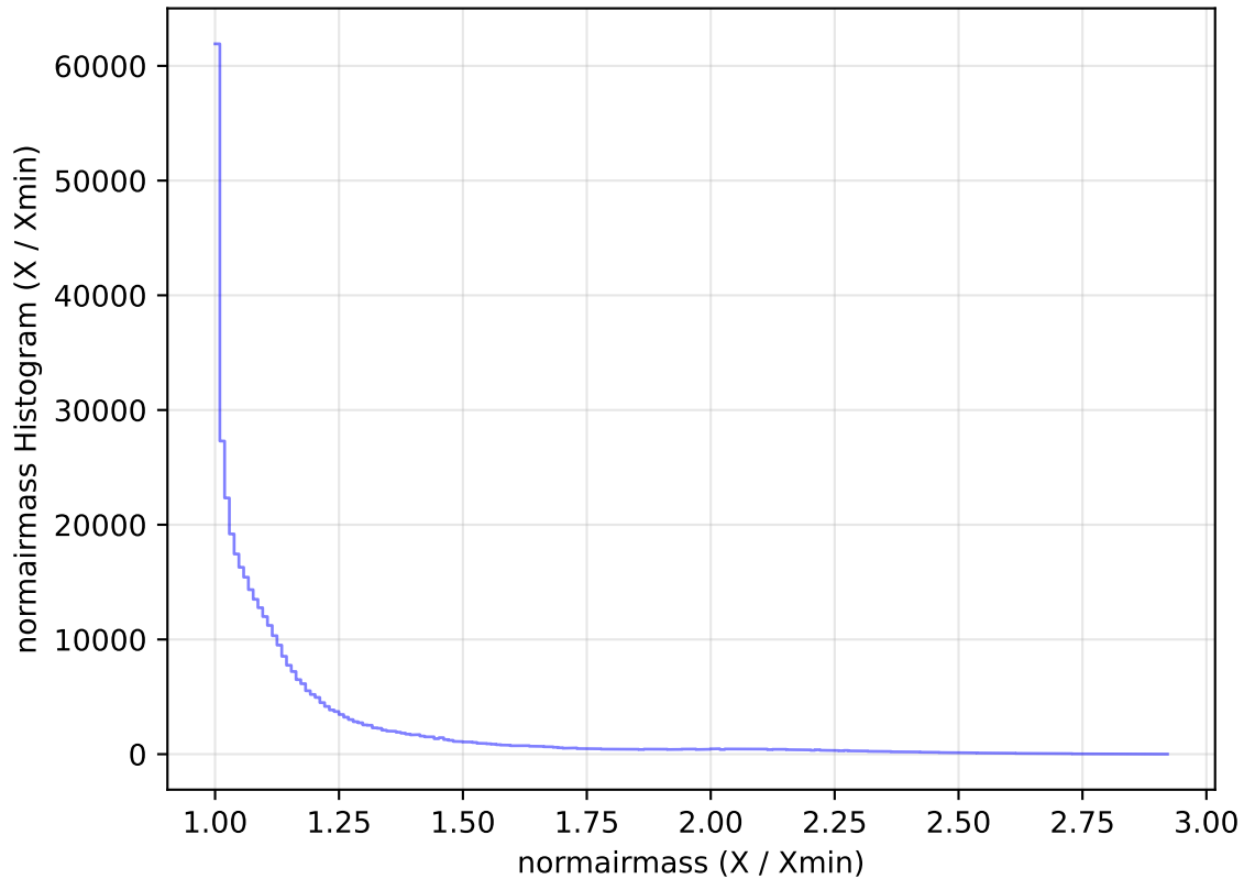
internal_u_expt27_nscale1.5v3.4_10yrs All sky z band: normairmass Histogram
