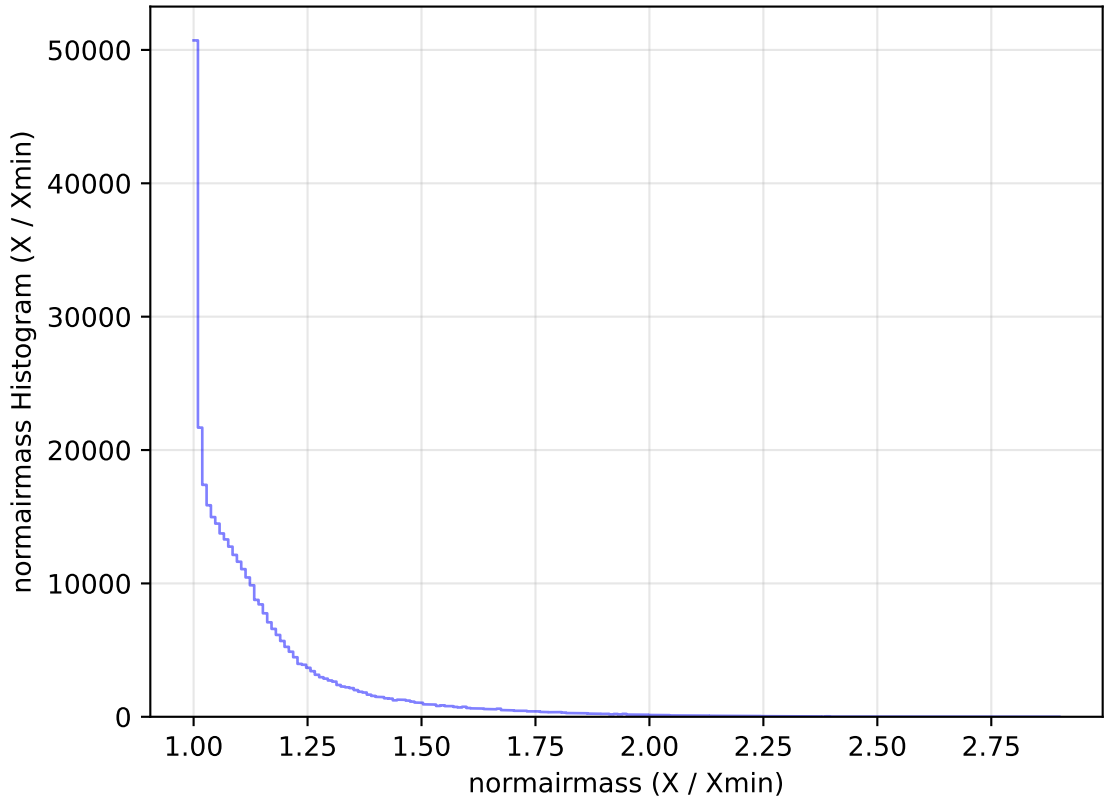
internal_u_expt27_nscale1.5v3.4_10yrs All sky y band: normairmass Histogram
