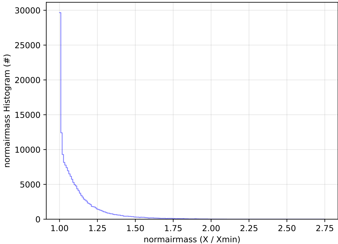
internal_u_expt27_nscale1.5v3.4_10yrs All sky u band: normairmass Histogram
