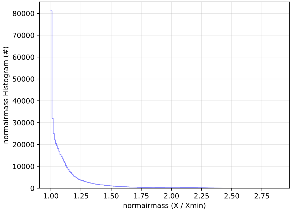
internal_u_expt27_nscale1.5v3.4_10yrs All sky r band: normairmass Histogram
