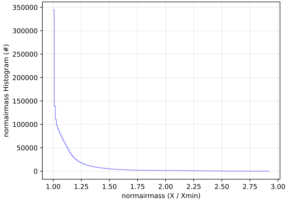
internal_u_expt27_nscale1.5v3.4_10yrs All sky all bands: normairmass Histogram
