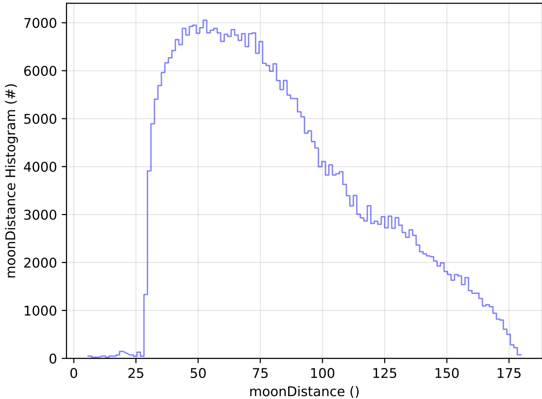
internal_u_expt27_nscale1.5v3.4_10yrs WFD z band: moonDistance Histogram
