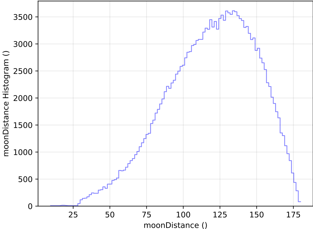
internal_u_expt27_nscale1.5v3.4_10yrs WFD u band: moonDistance Histogram
