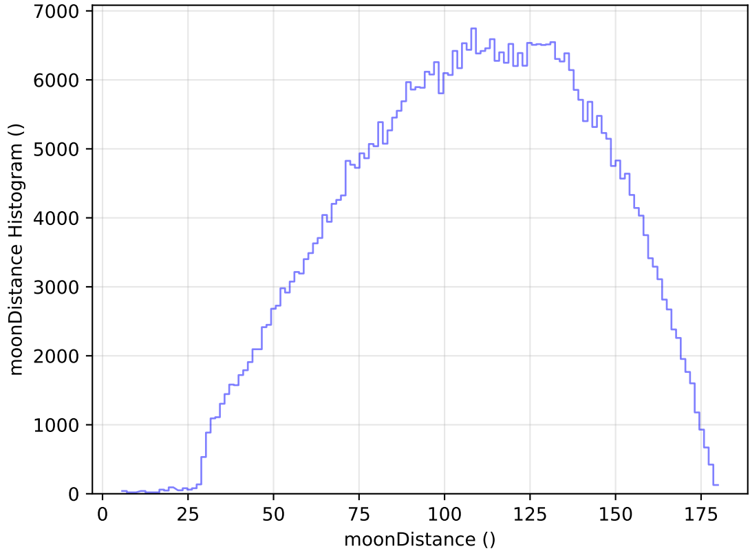
internal_u_expt27_nscale1.5v3.4_10yrs WFD r band: moonDistance Histogram
