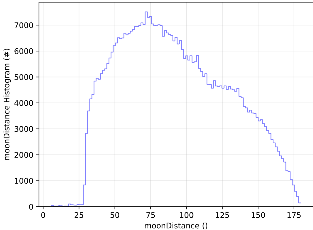
internal_u_expt27_nscale1.5v3.4_10yrs WFD i band: moonDistance Histogram
