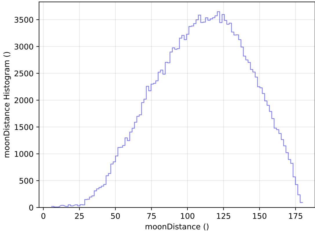
internal_u_expt27_nscale1.5v3.4_10yrs WFD g band: moonDistance Histogram
