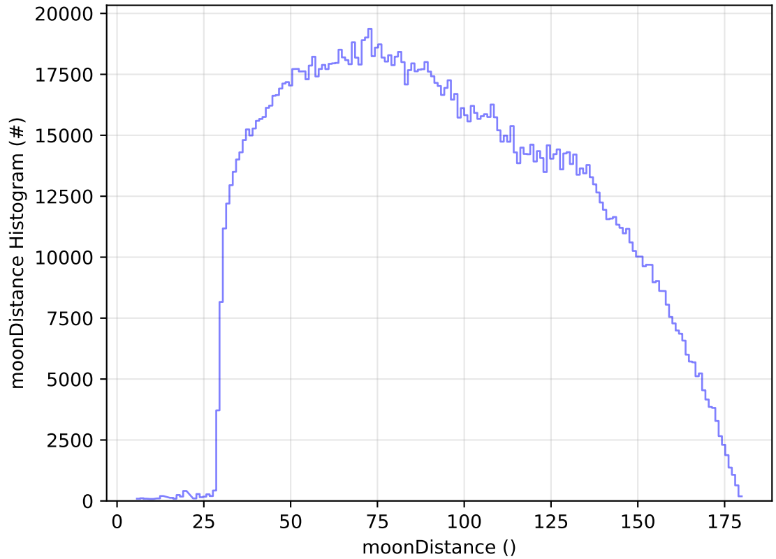
internal_u_expt27_nscale1.5v3.4_10yrs WFD all bands: moonDistance Histogram
