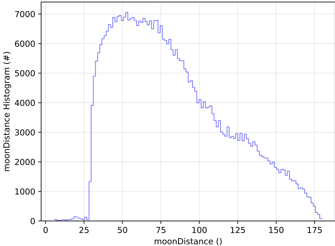
internal_u_expt27_nscale1.5v3.4_10yrs All sky z band: moonDistance Histogram
