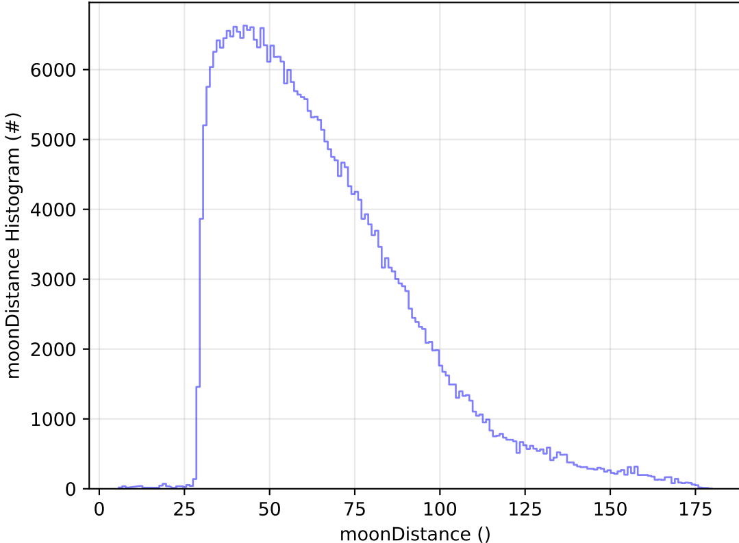
internal_u_expt27_nscale1.5v3.4_10yrs All sky y band: moonDistance Histogram
