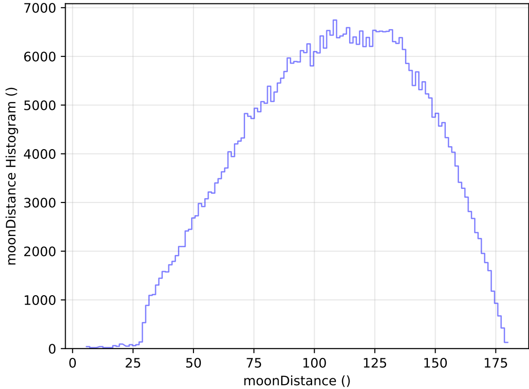
internal_u_expt27_nscale1.5v3.4_10yrs All sky r band: moonDistance Histogram
