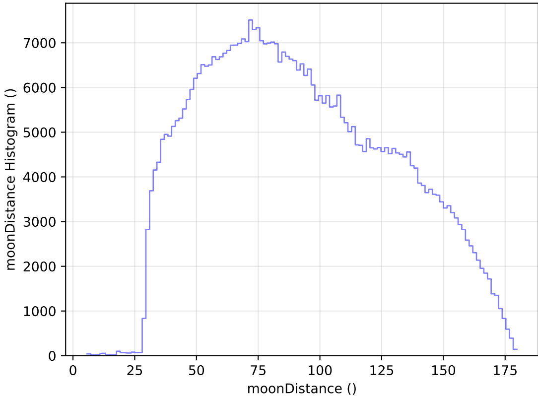
internal_u_expt27_nscale1.5v3.4_10yrs All sky i band: moonDistance Histogram
