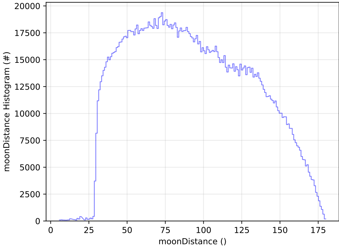
internal_u_expt27_nscale1.5v3.4_10yrs All sky all bands: moonDistance Histogram
