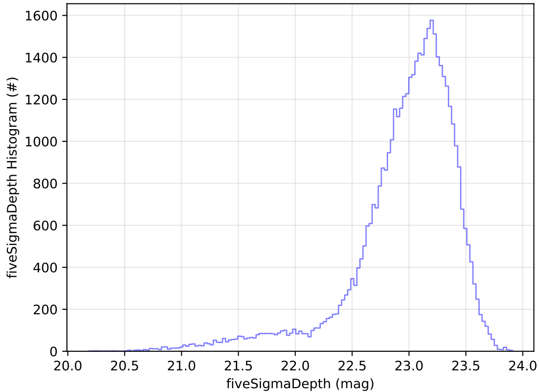
internal_u_expt27_nscale1.5v3.4_10yrs Yr 1 z band: fiveSigmaDepth Histogram
