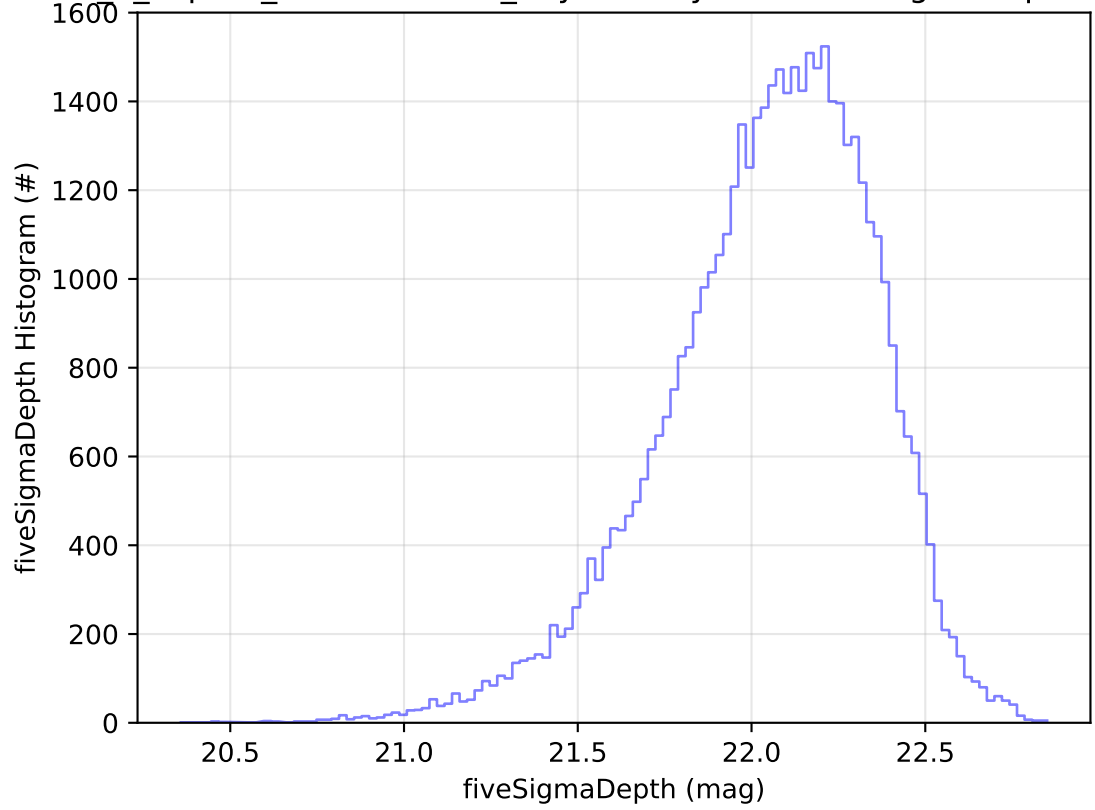
internal_u_expt27_nscale1.5v3.4_10yrs Yr 1 y band: fiveSigmaDepth Histogram
