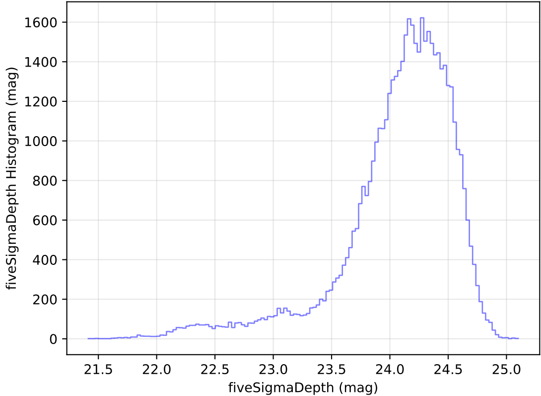
internal_u_expt27_nscale1.5v3.4_10yrs Yr 1 r band: fiveSigmaDepth Histogram
