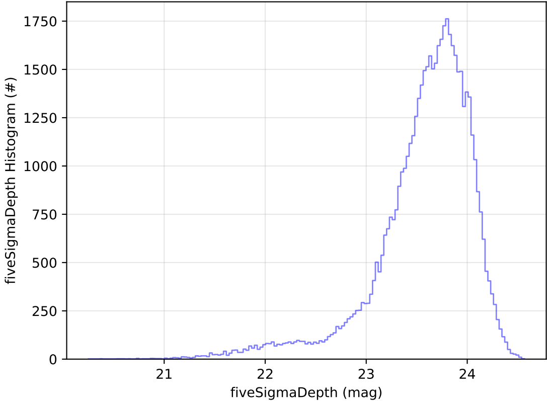
internal_u_expt27_nscale1.5v3.4_10yrs Yr 1 i band: fiveSigmaDepth Histogram
