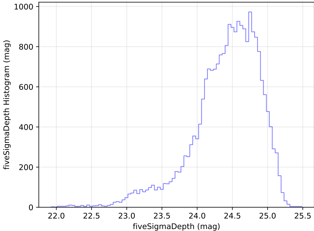
internal_u_expt27_nscale1.5v3.4_10yrs Yr 1 g band: fiveSigmaDepth Histogram
