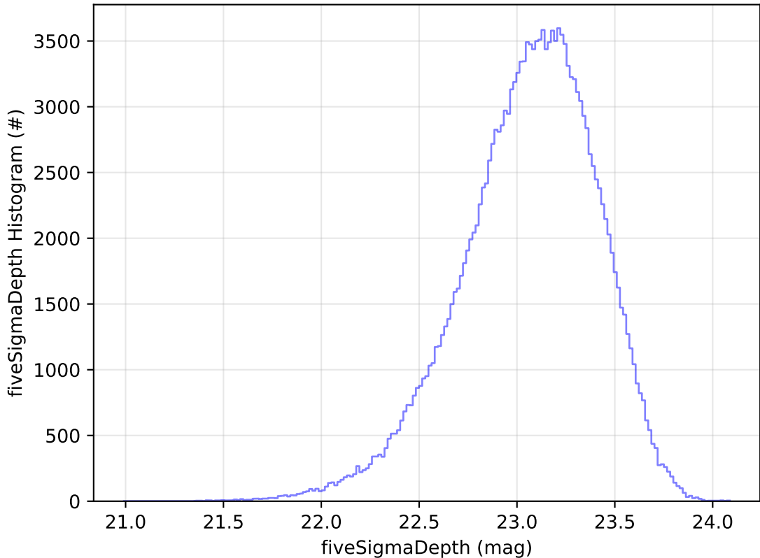
internal_u_expt27_nscale1.5v3.4_10yrs WFD u band: fiveSigmaDepth Histogram
