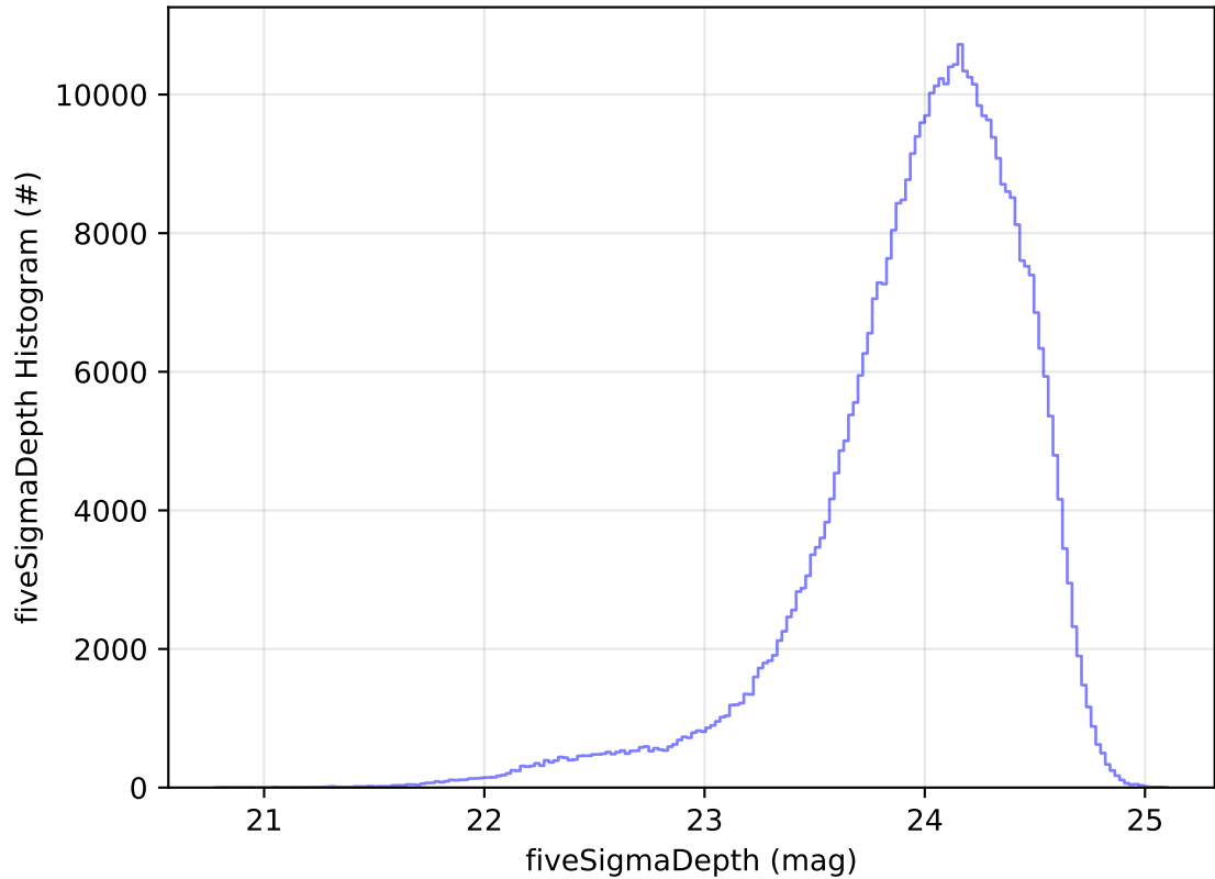
internal_u_expt27_nscale1.5v3.4_10yrs WFD r band: fiveSigmaDepth Histogram
