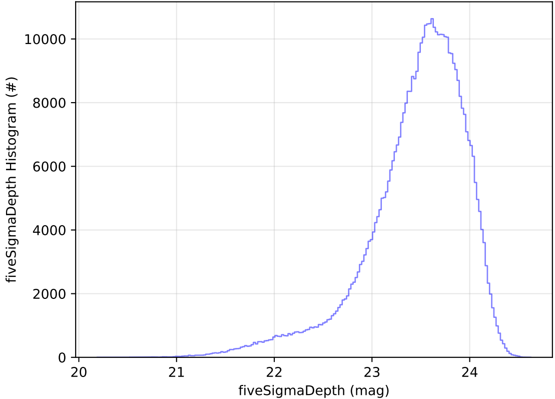
internal_u_expt27_nscale1.5v3.4_10yrs WFD i band: fiveSigmaDepth Histogram
