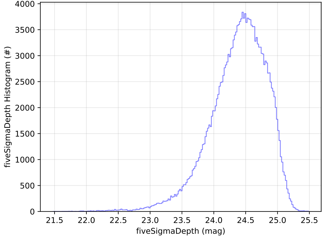
internal_u_expt27_nscale1.5v3.4_10yrs WFD g band: fiveSigmaDepth Histogram
