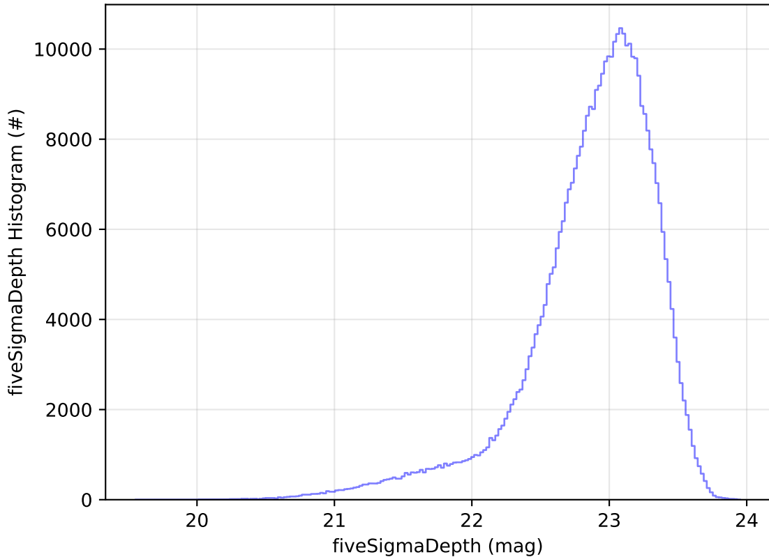
internal_u_expt27_nscale1.5v3.4_10yrs All sky z band: fiveSigmaDepth Histogram
