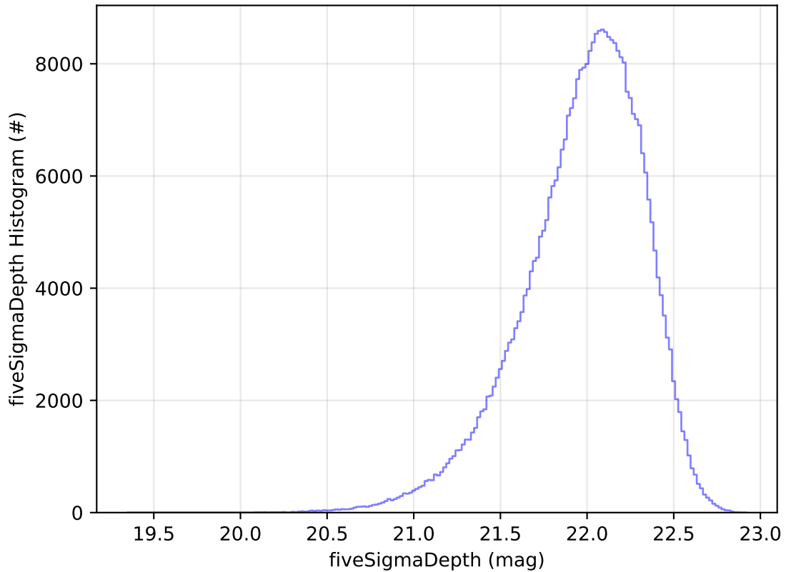
internal_u_expt27_nscale1.5v3.4_10yrs All sky y band: fiveSigmaDepth Histogram
