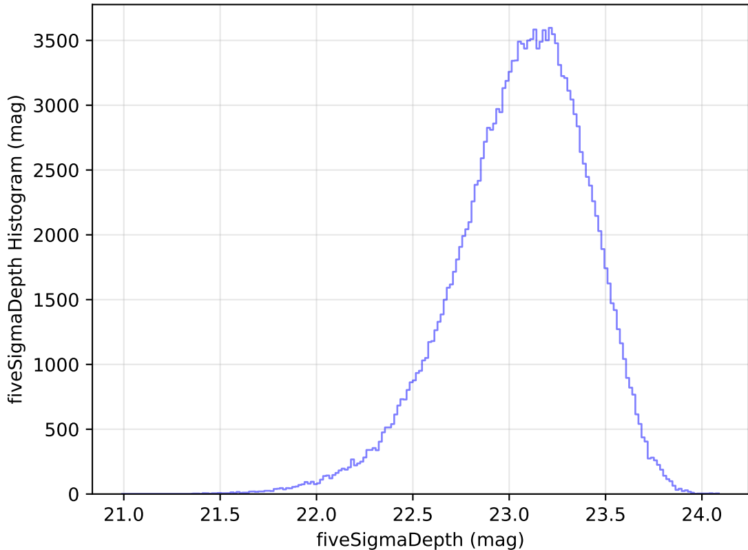
internal_u_expt27_nscale1.5v3.4_10yrs All sky u band: fiveSigmaDepth Histogram
