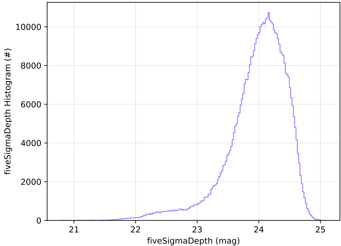
internal_u_expt27_nscale1.5v3.4_10yrs All sky r band: fiveSigmaDepth Histogram
