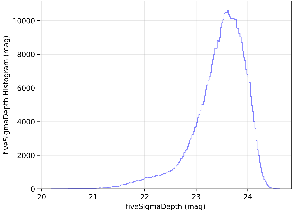
internal_u_expt27_nscale1.5v3.4_10yrs All sky i band: fiveSigmaDepth Histogram
