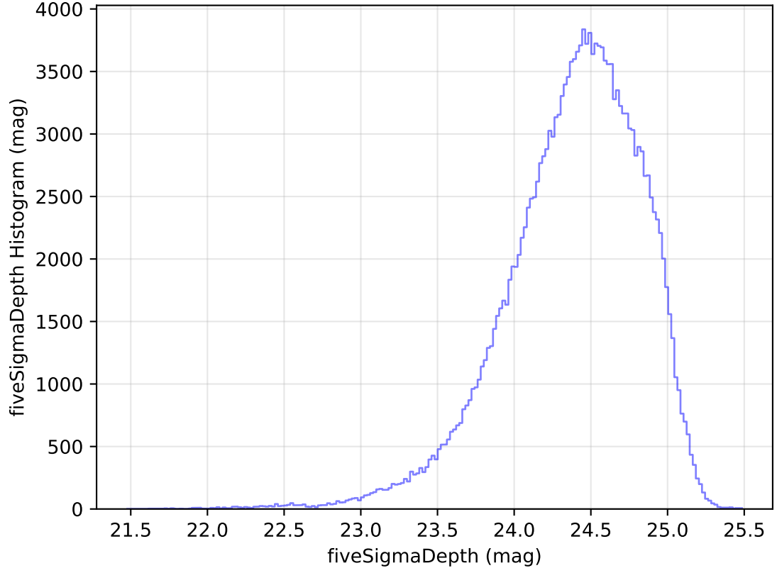
internal_u_expt27_nscale1.5v3.4_10yrs All sky g band: fiveSigmaDepth Histogram
