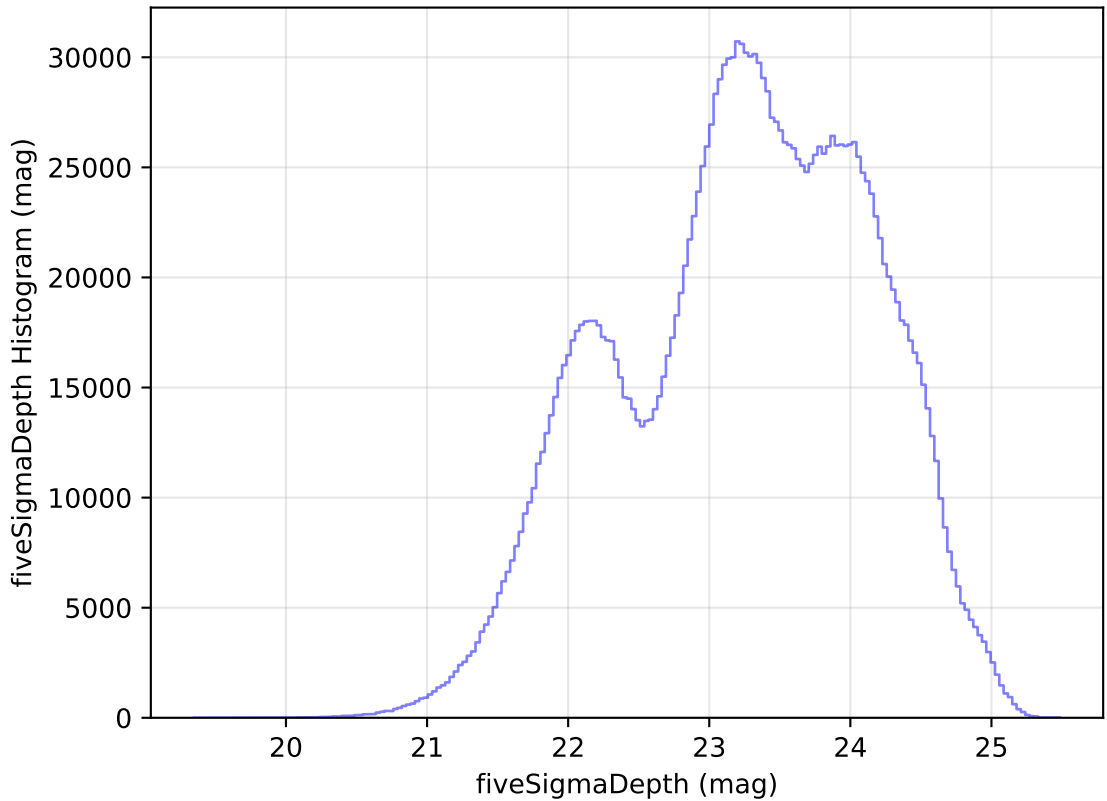
internal_u_expt27_nscale1.5v3.4_10yrs All sky all bands: fiveSigmaDepth Histogram
