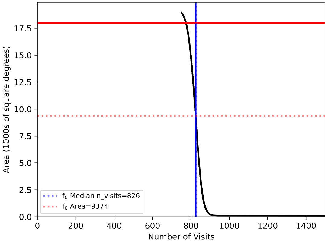
internal_u_expt27_nscale1.5v3.4_10yrs WFD: fO
