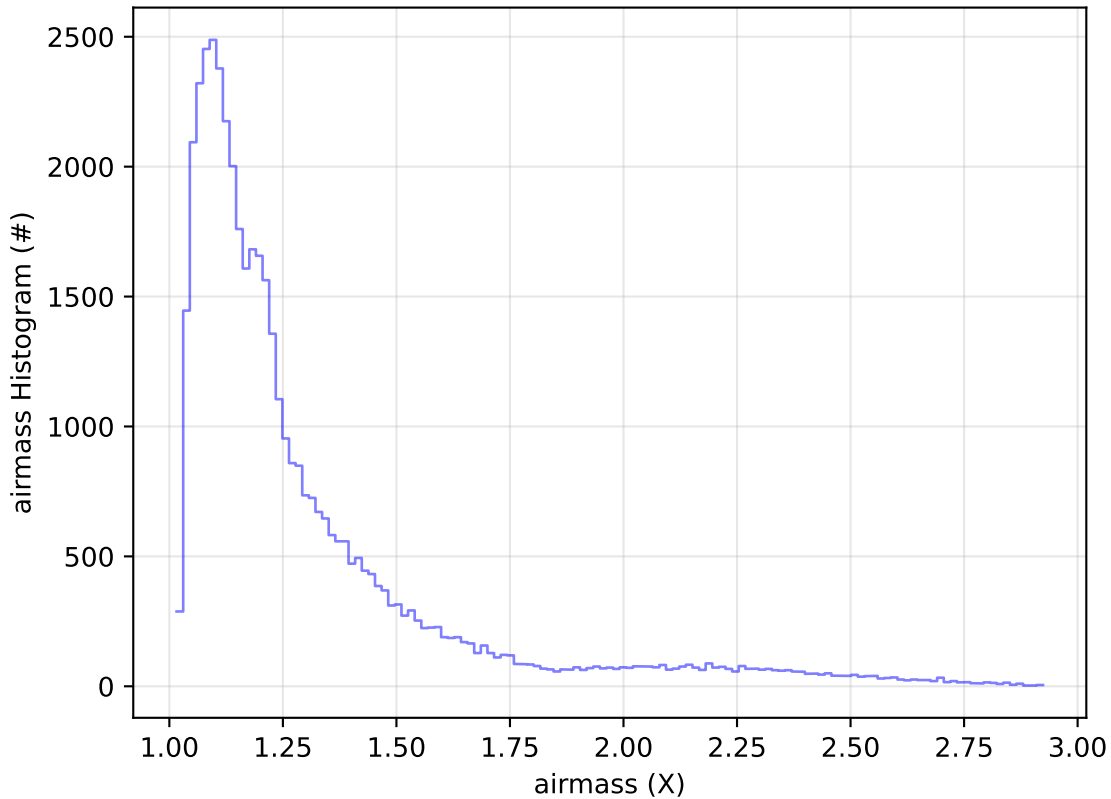
internal_u_expt27_nscale1.5v3.4_10yrs Yr 1 z band: airmass Histogram
