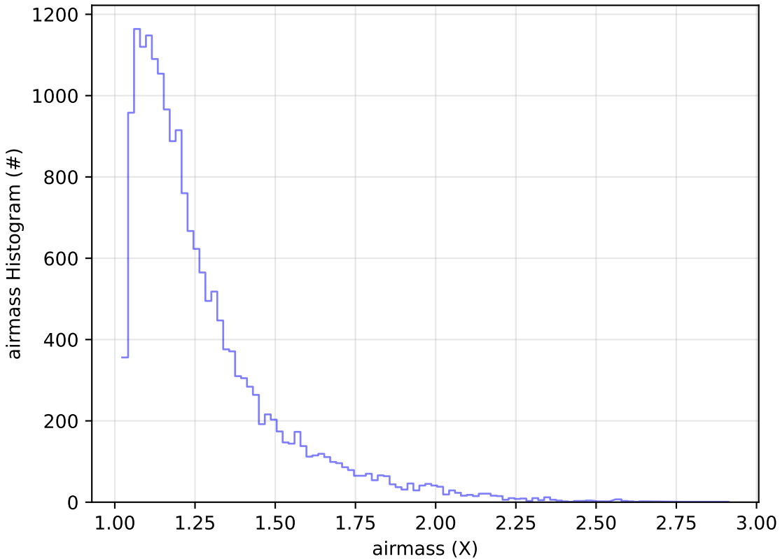
internal_u_expt27_nscale1.5v3.4_10yrs Yr 1 u band: airmass Histogram
