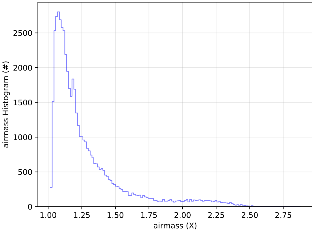
internal_u_expt27_nscale1.5v3.4_10yrs Yr 1 r band: airmass Histogram
