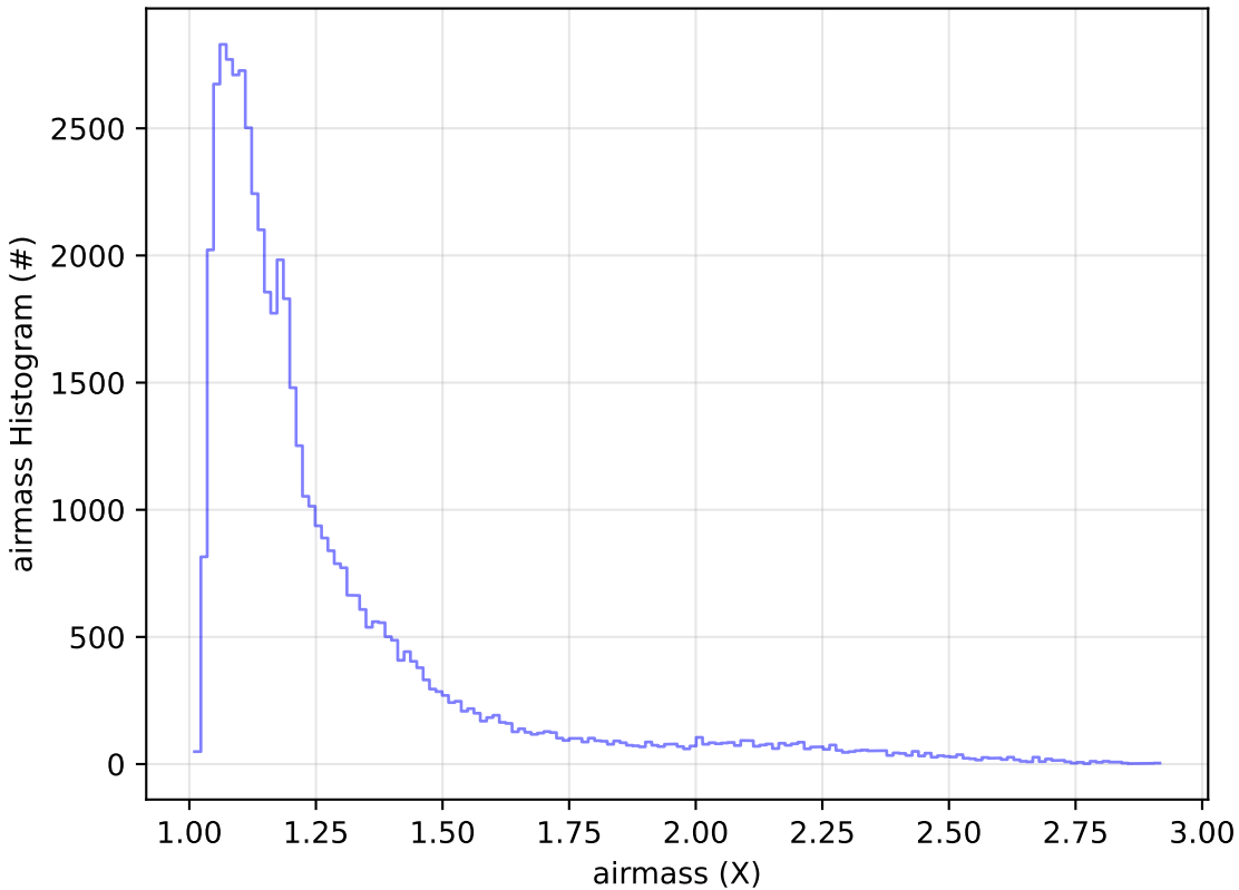
internal_u_expt27_nscale1.5v3.4_10yrs Yr 1 i band: airmass Histogram
