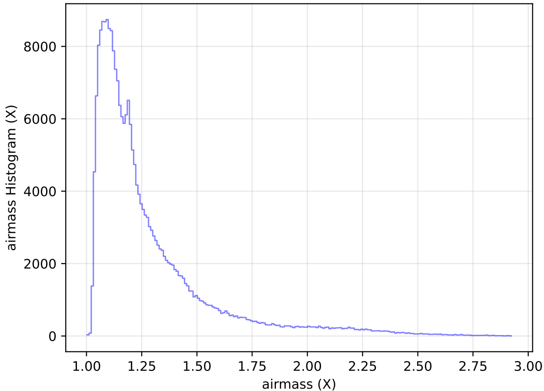
internal_u_expt27_nscale1.5v3.4_10yrs Yr 1 all bands: airmass Histogram
