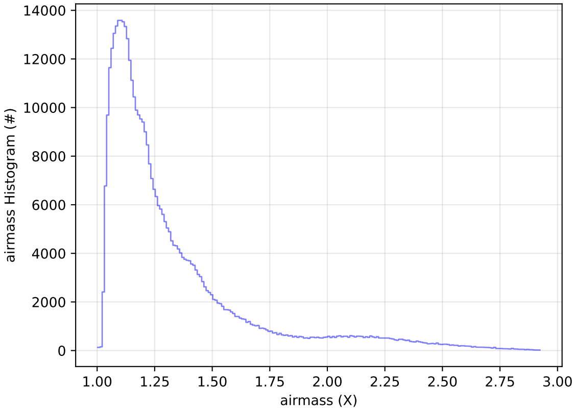
internal_u_expt27_nscale1.5v3.4_10yrs WFD z band: airmass Histogram
