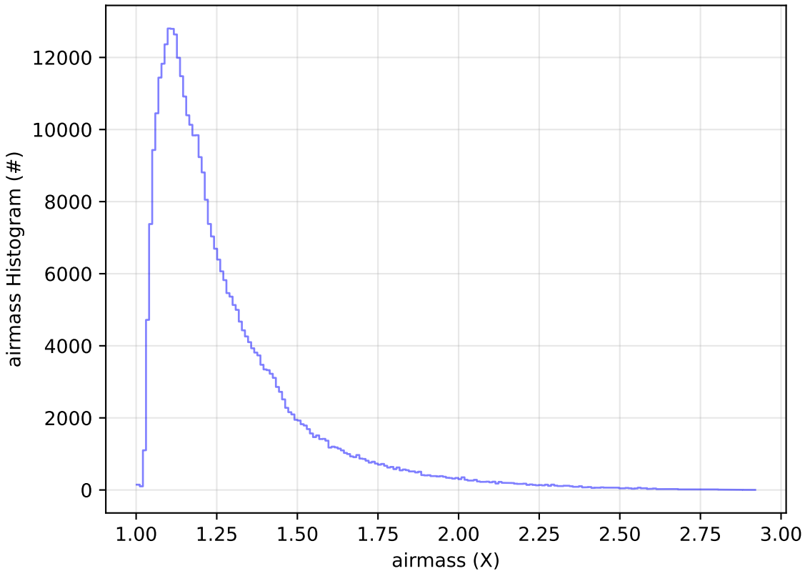
internal_u_expt27_nscale1.5v3.4_10yrs WFD y band: airmass Histogram
