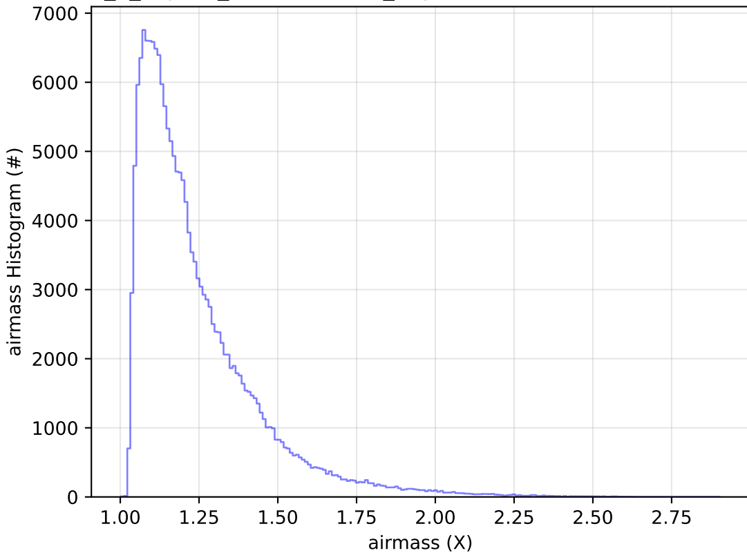
internal_u_expt27_nscale1.5v3.4_10yrs WFD u band: airmass Histogram
