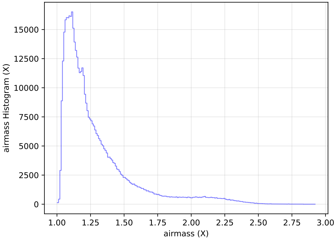
internal_u_expt27_nscale1.5v3.4_10yrs WFD r band: airmass Histogram
