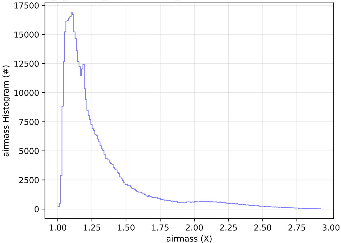
internal_u_expt27_nscale1.5v3.4_10yrs WFD i band: airmass Histogram
