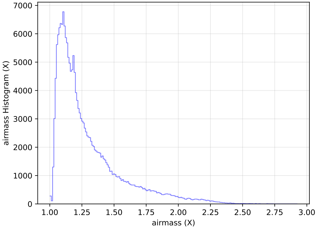
internal_u_expt27_nscale1.5v3.4_10yrs WFD g band: airmass Histogram
