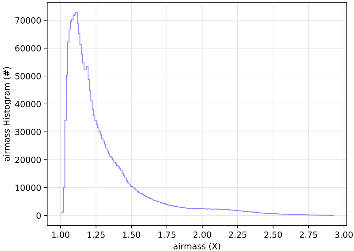
internal_u_expt27_nscale1.5v3.4_10yrs WFD all bands: airmass Histogram
