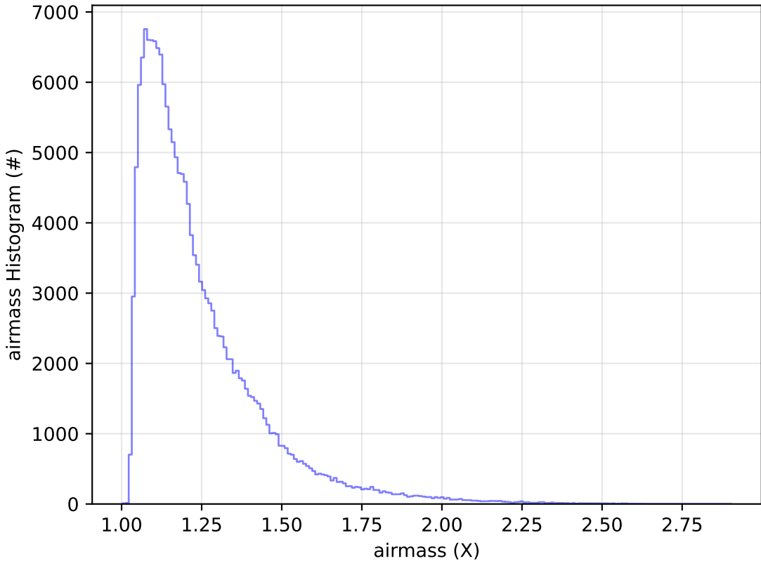
internal_u_expt27_nscale1.5v3.4_10yrs All sky u band: airmass Histogram
