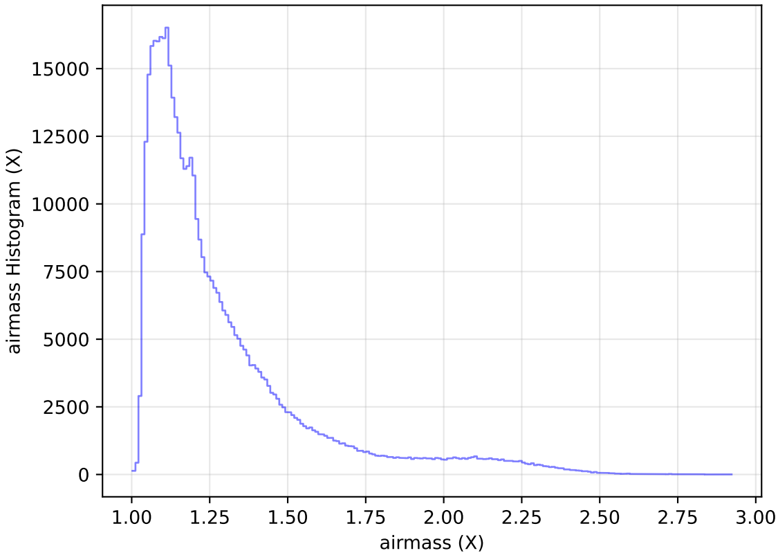
internal_u_expt27_nscale1.5v3.4_10yrs All sky r band: airmass Histogram
