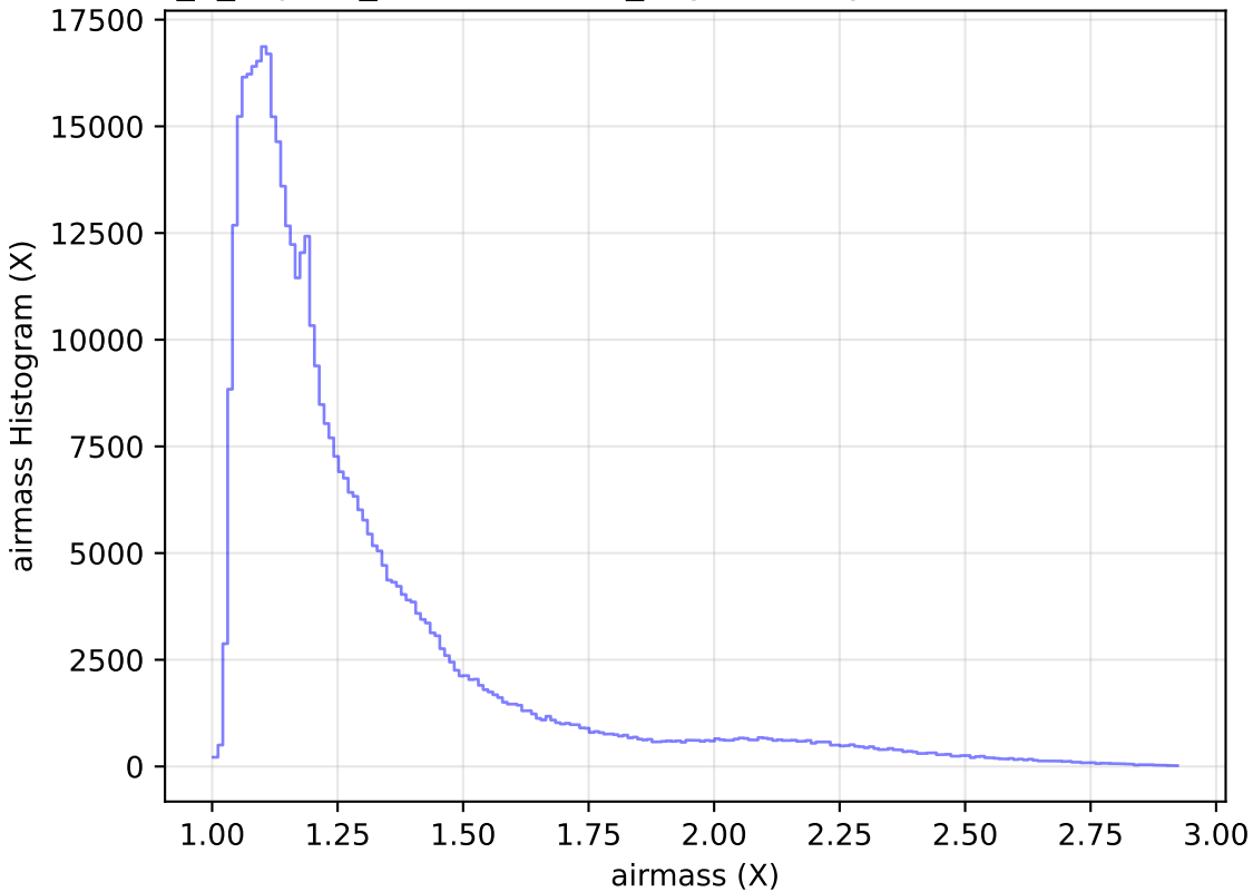
internal_u_expt27_nscale1.5v3.4_10yrs All sky i band: airmass Histogram
