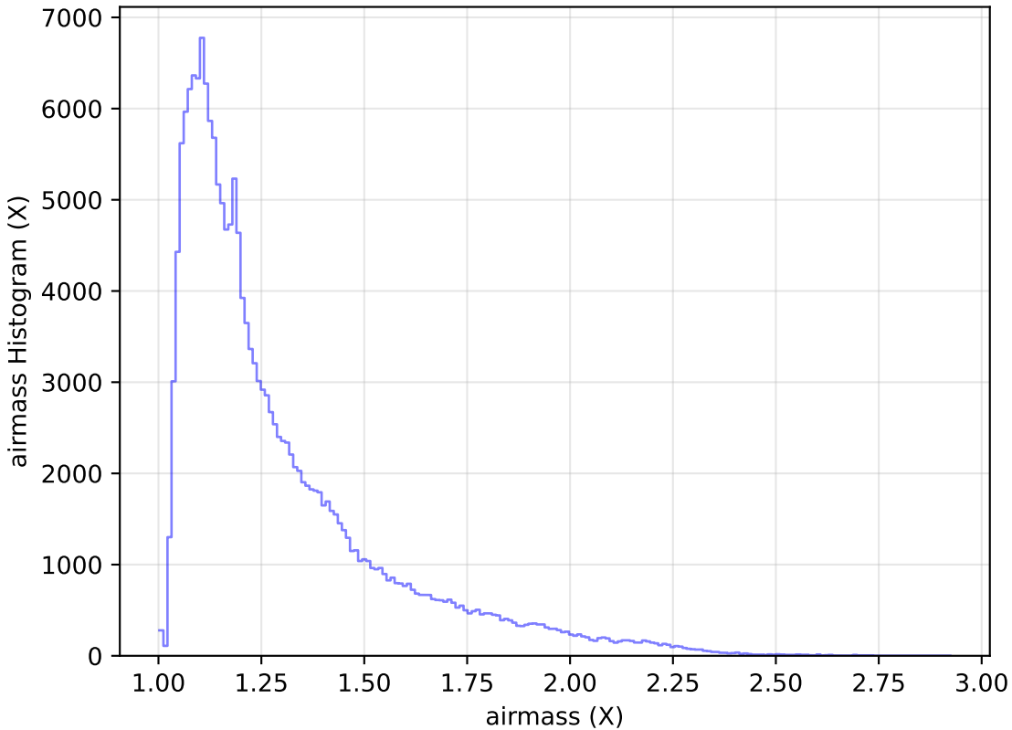
internal_u_expt27_nscale1.5v3.4_10yrs All sky g band: airmass Histogram
